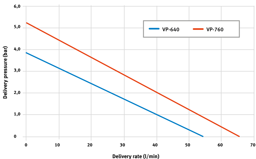
PUMP CURVES WT4-90
